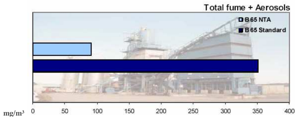
Figure 4 Testing at Mixing Plant B 65 versus B 65 with aspha-min®
